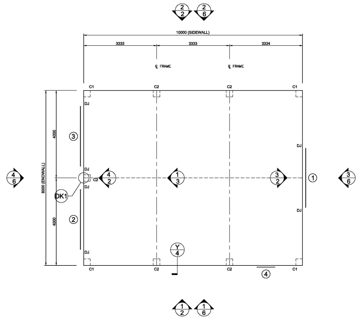
1 FOUNDATION PLAN AND MEMBER LAYOUT SCALE: 1 = 100
