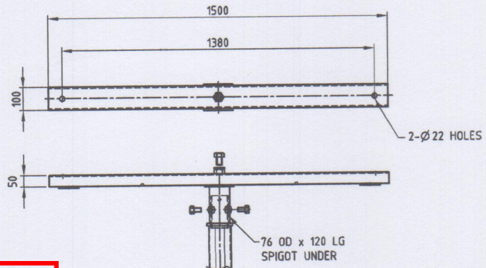
DETAIL 1 SCALE 1:15
