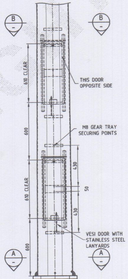
DETAIL 2 SCALE 1:15
