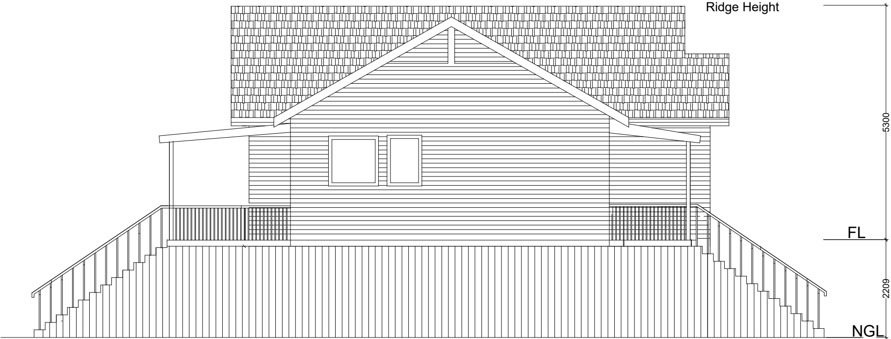
EAST ELEVATION
