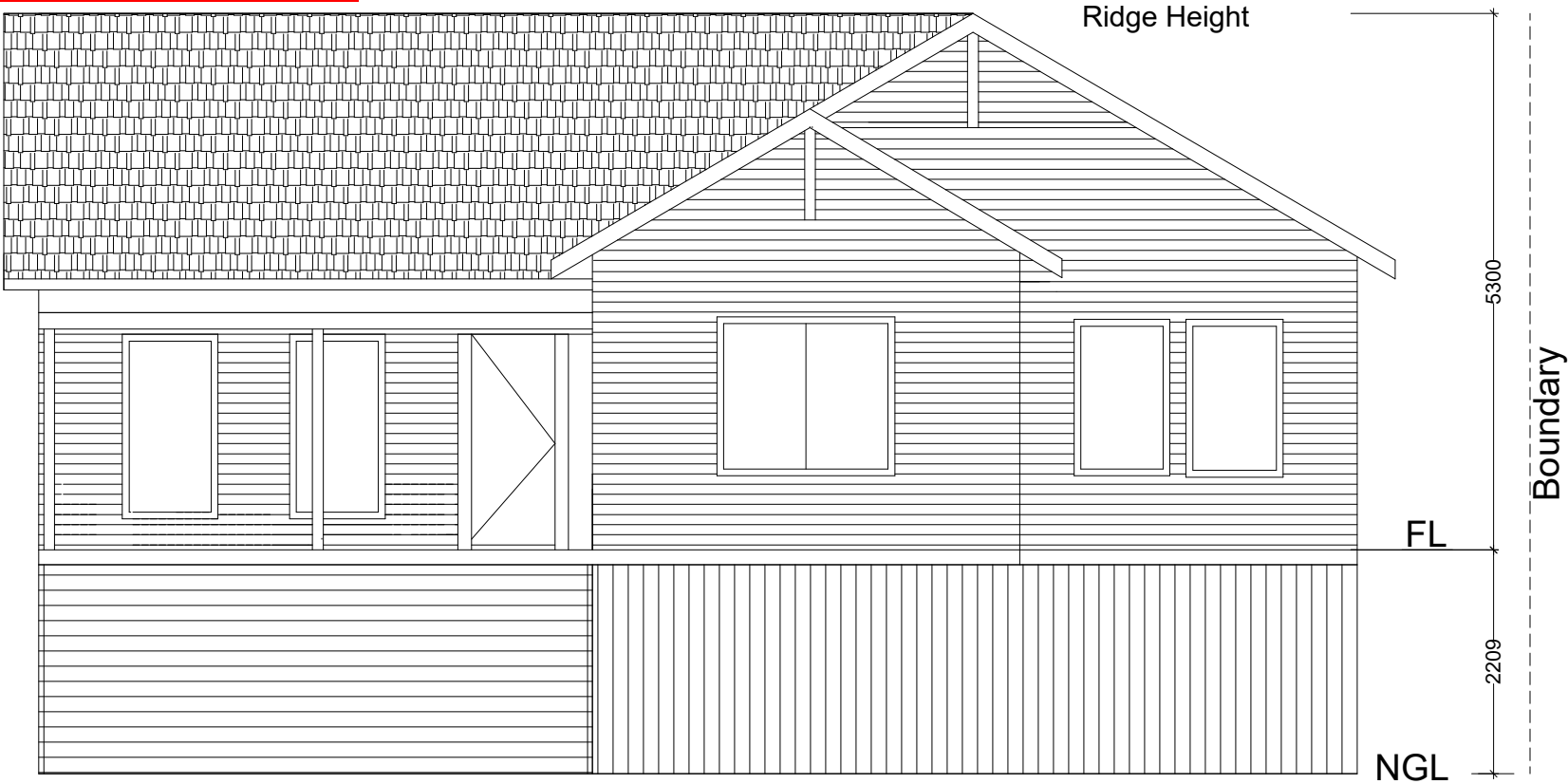
NORTH ELEVATION
