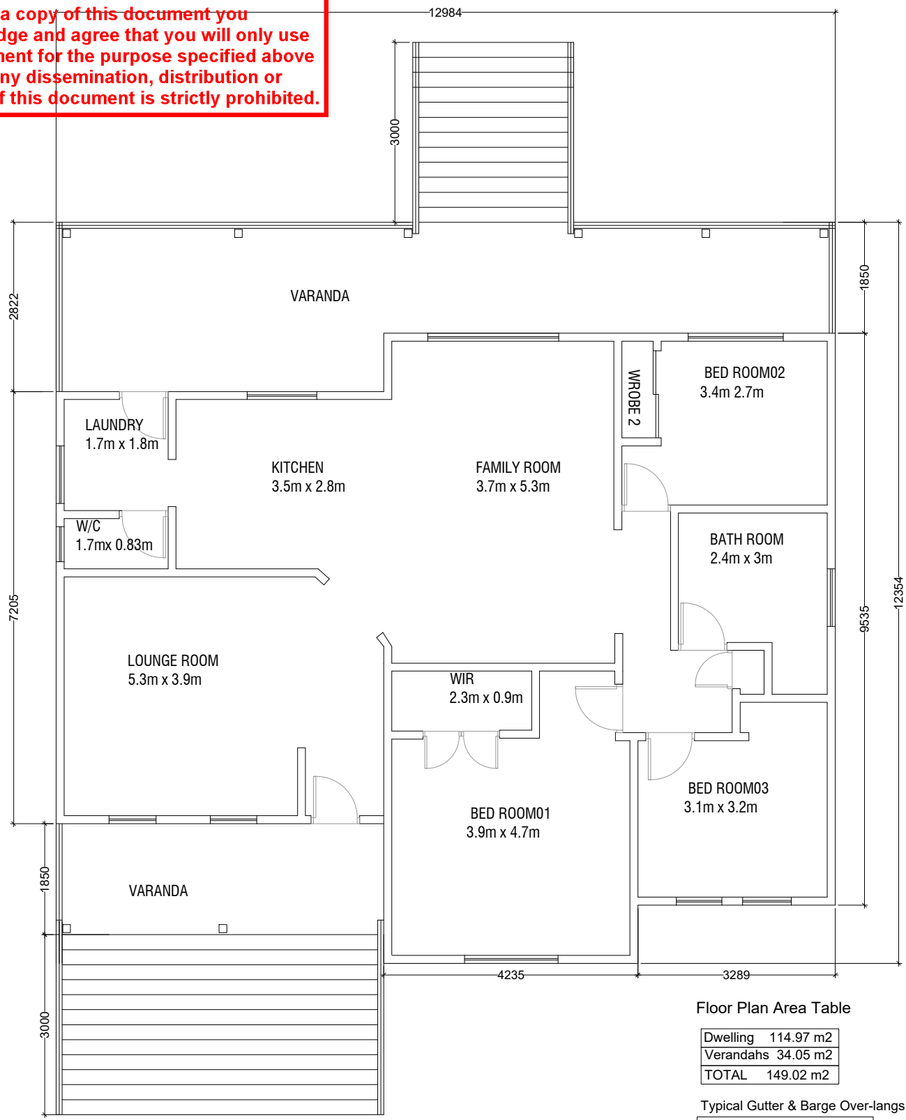
Floor Plan
