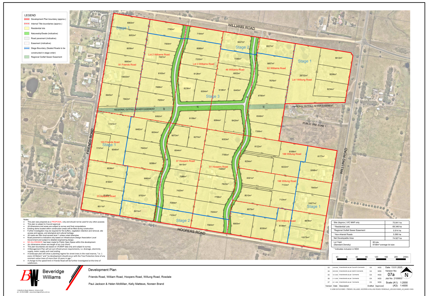
Figure 5: Subdivision Plan
