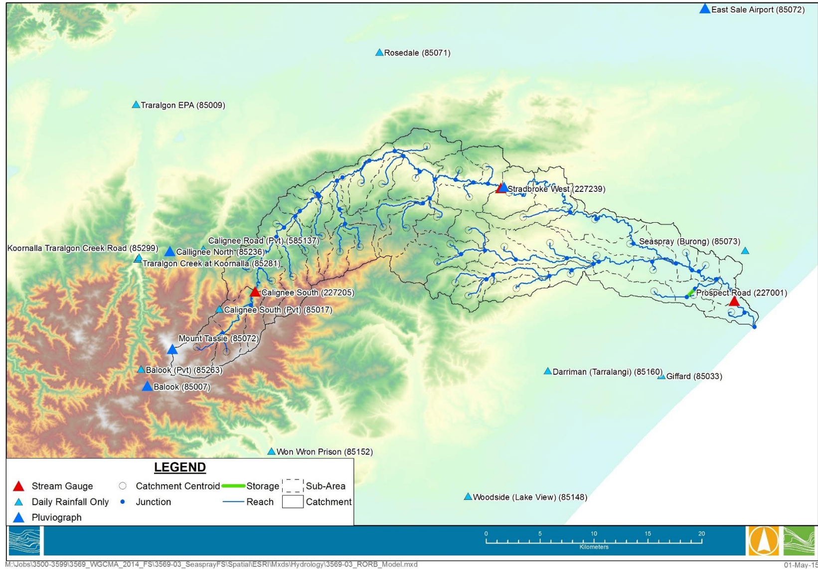
Figure 4-1 RORB Model Structure
