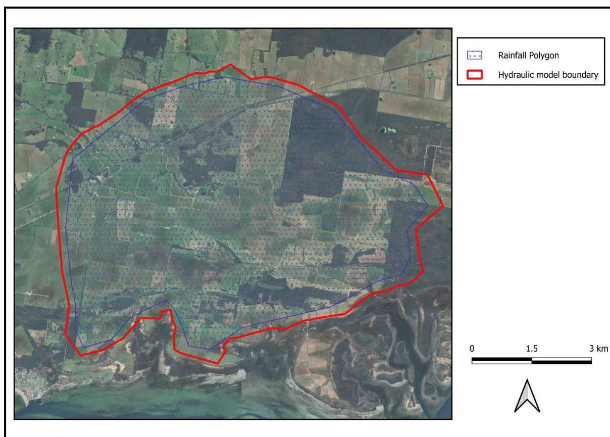
Figure 3-8 Rainfall polygon extent
