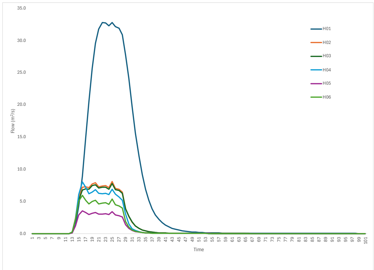
Figure 2-7 Modelled flows at each of the six print nodes for the AEP 1% storm
