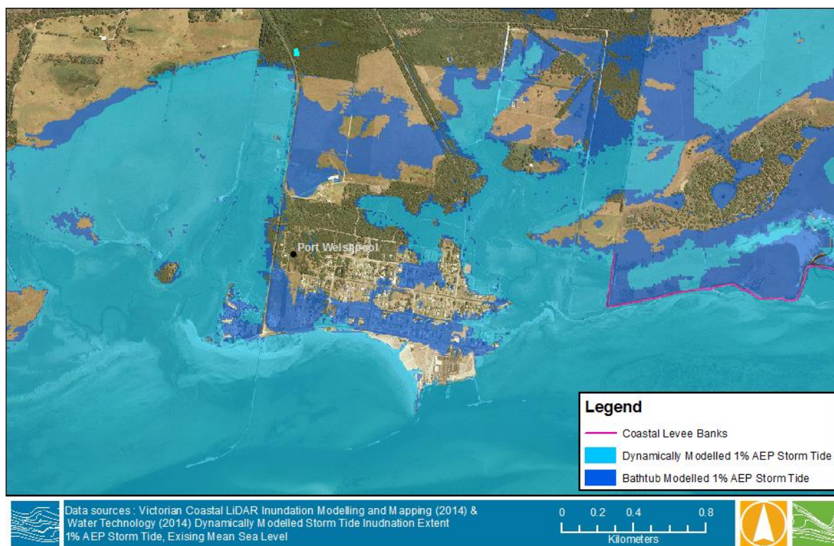
Figure 5-9 Comparison of the 1% AEP Storm Tide under Existing MSL, Modelled Using the Bathtub Technique and a Dynamic Hydrodynamic Model – Port Welshpool
