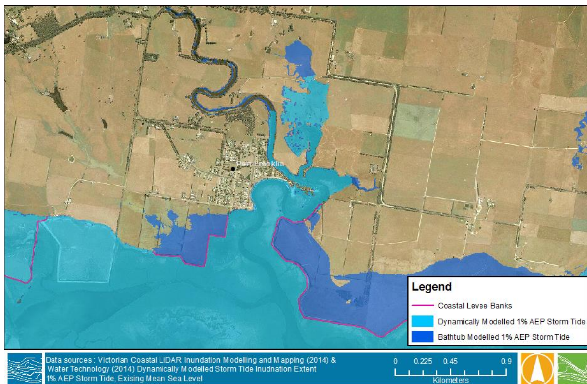
Figure 5-8 Comparison of the 1% AEP Storm Tide under Existing MSL, Modelled Using the Bathtub Technique and a Dynamic Hydrodynamic Model – Port Franklin (Note: This figure does not show inundation extents from riverine flooding from the Franklin River).
