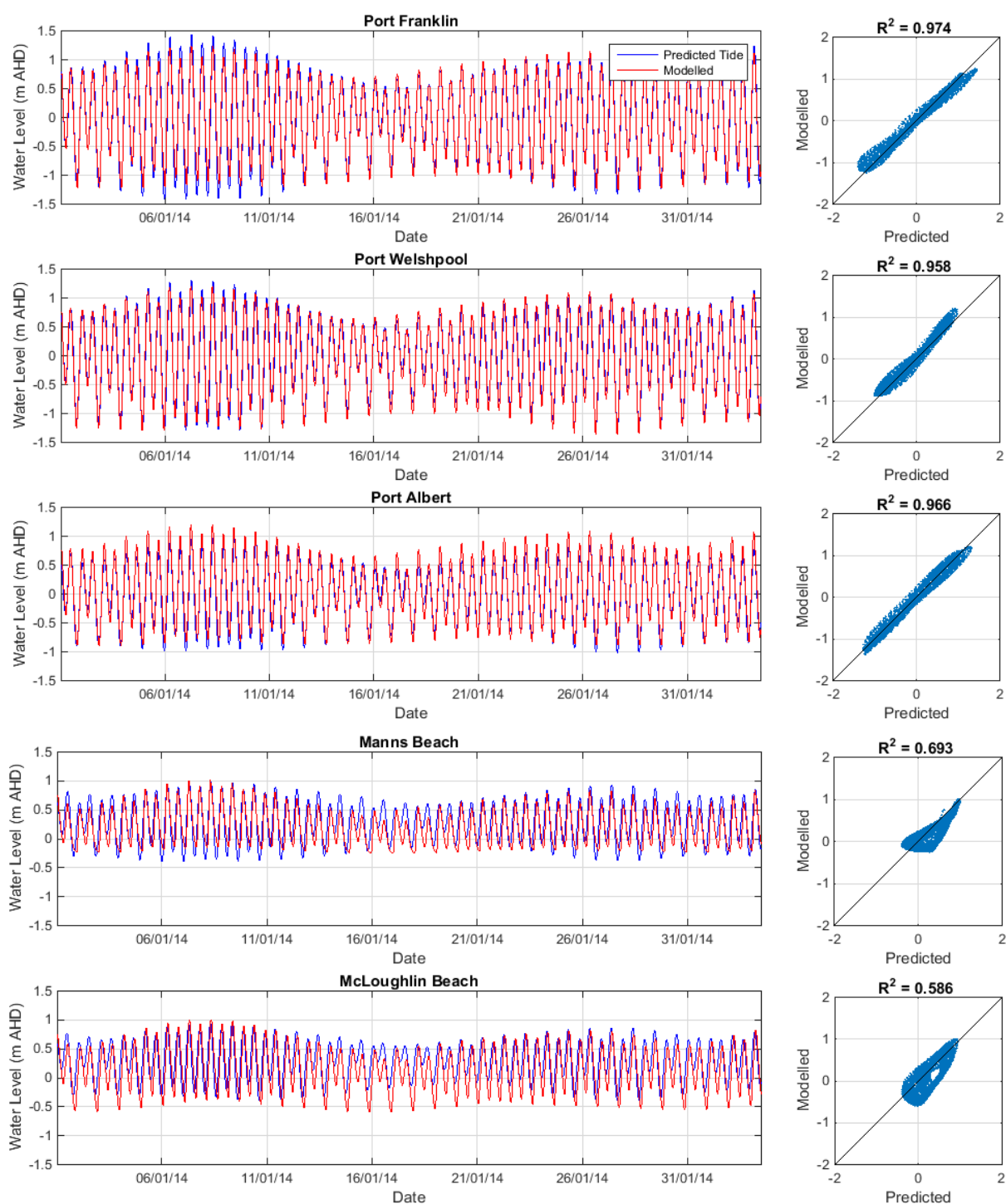
Figure 4-4 Astronomical Tidal Water Level Calibration
